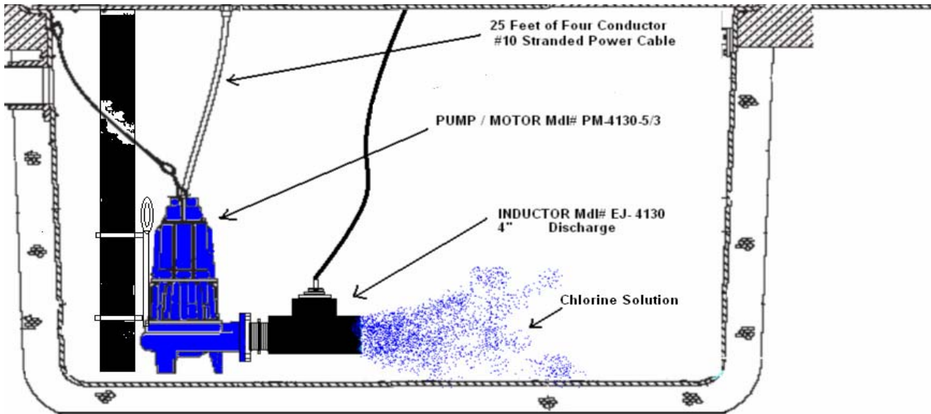
Global Treat, Inc. SWEET Package Induction System Model # MEGA-SWEET-4130-5/3
